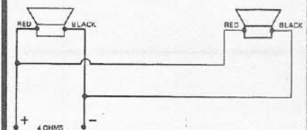
FIGURE 11 Connection of 2 EVM-12L Speakers in Parallel
