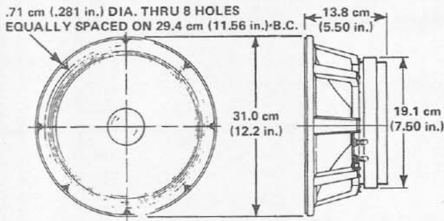
FIGURE 1 – Dimensions
